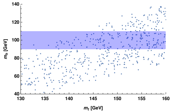
FIG. 1. m_h versus m_t (at \mu \sim f_\pi ), with the blue stripe highlighting the correct Higgs mass m_h \in [90, 110] [38].
