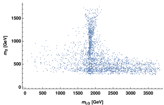
FIG. 2. m_S versus m_{LQ} . See text for details.
