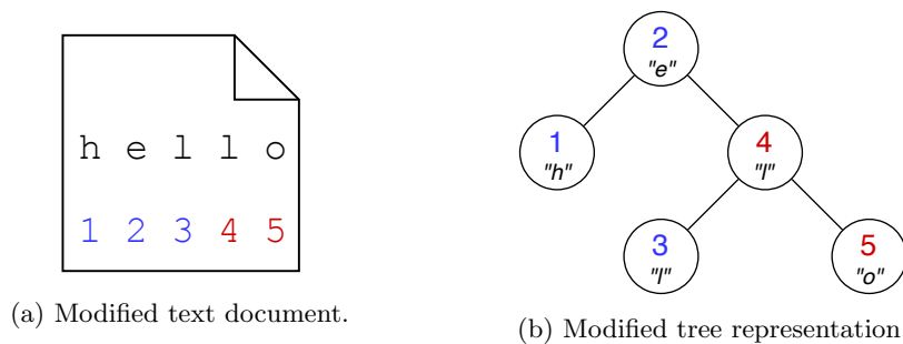
Fig. 5: A text document and its tree representation. Red numbers indicate index changes compared to Figure 4.
