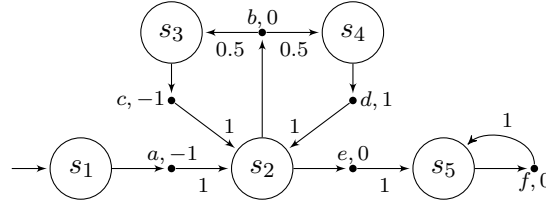
Figure 5: There exists a strategy \sigma ensuring AS_{\mathcal{M},s_1}^\sigma[\text{DBW}_{\text{mp}}] but it requires infinite memory as it needs to use b up to the point where the running sum becomes non-negative, then switch to e .
