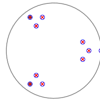
Fig. 1. The eigenvalues \lambda_w (plotted as red \times 's) of the embedding system coincide with the products (plotted as blue o 's) of up to d eigenvalues of the linear subsystem \mathcal{B}(\lambda) . + — eigenvalues \lambda , dotted line — unit circle.
