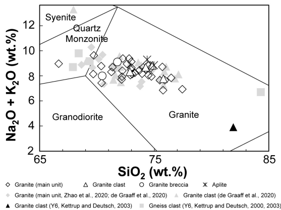
Figure 2. Total alkalis versus \text{SiO}_2 (TAS) diagram.
