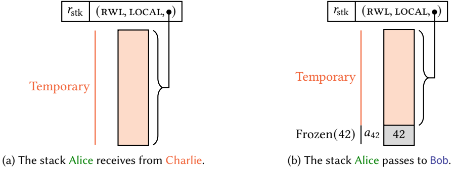
Fig. 8. A scenario where a stack capability is passed in a register r_{\text{stk}} between different parties.
