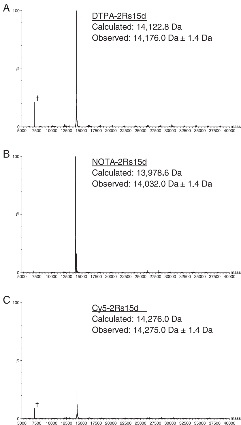
Figure 4. The purified sdAb-conjugates CHX-A"-DTPA-2Rs15d (A), NOTA-2Rs15d (B) and Cy5-2Rs15d (C) are homogeneous single-conjugated sdAbs. Unreacted sdAb (14,430.0 Da), SrtA (22,133.9 Da) and the acyl-enzyme intermediate (35,182.5 Da) are absent in the ESI-Q-ToF deconvoluted mass spectra. In (A) and (B), complexation of Fe by the chelating agents is seen (net change in calculated mass of +52.8 Da). However, this did not interfere with further radiolabeling. (†: Peak arising from artifact in deconvolution)
