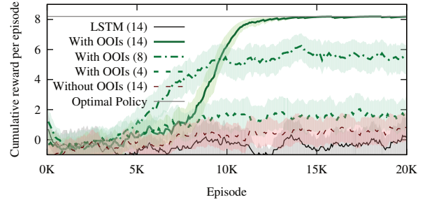
Figure 7: Cumulative reward per episode obtained on TreeMaze, using 14, 8 or 4 options. Even with an insufficient amount of options (8 or 4), OOIs lead to better performance than no OOIs but 14 options. LSTM over options learns the task after more than 100K episodes (not shown).
