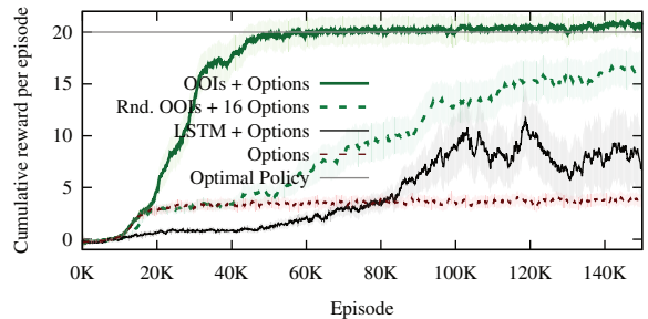
Figure 5: Cumulative reward per episode obtained on modified DuplicatedInput, with random or designed OOIs, without OOIs and using an LSTM over options. Despite our efforts, an LSTM over options repeatedly learns then forgets optimal policies, as shown by the high variance of its line.
