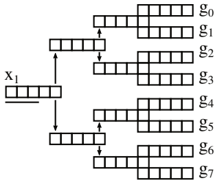
Figure 6: TreeMaze environment. The agent starts at x_1 and must go to one of the leaves. The leaf to be reached is indicated by 3 bits observed at time-steps 1, 2 and 3.
