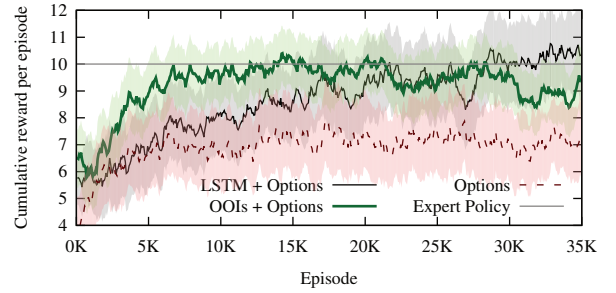
Figure 4: Cumulative reward per episode obtained on our object gathering task, with OOIs, without OOIs, and using an LSTM over options. OOIs learns an expert-level policy much quicker than an LSTM over options. The LSTM curve flattens-out (with high variance) after about 30K episodes.
